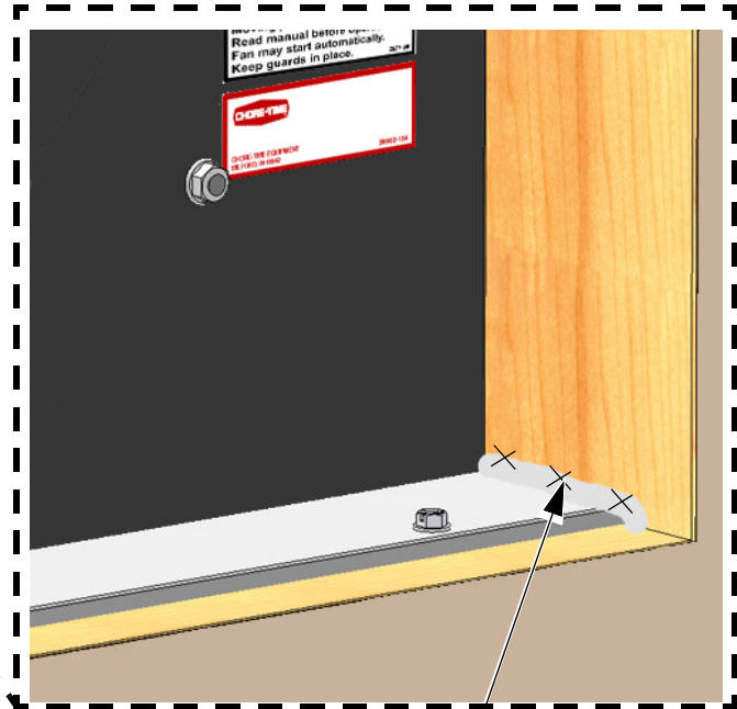
Caulk Both Ends of the Bottom Shelf
