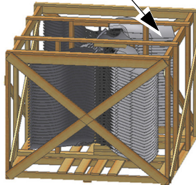
Fan Blade Package (53219-XX, 56494-XX, 54529-XX, 56108-XX, or 57022-XX)
